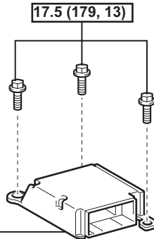
CENTER AIRBAG SENSOR ASSEMBLY
