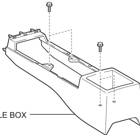
PARKING BRAKE HOLE COVER SUB-ASSEMBLY
